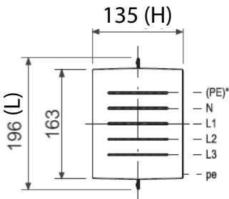
Section dimensions*
